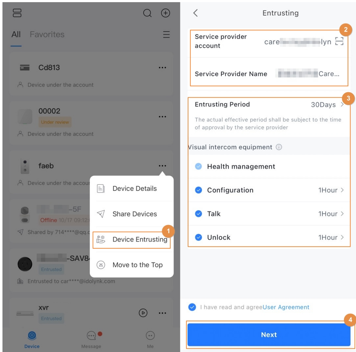
Figure 4-14 Entrust a device
