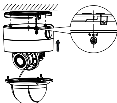
Figure 2-21 Fix Camera to Base Plate
