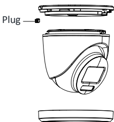
Figure 2-11 Take Apart Base and Main Body
