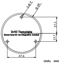
Figure 2. 1 Drill Template
