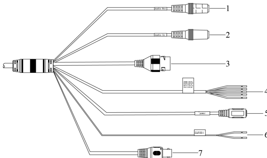
Figure 2-2 Cable ports
