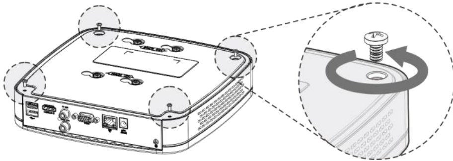
Figure 1-1 Installing HDD (1)
