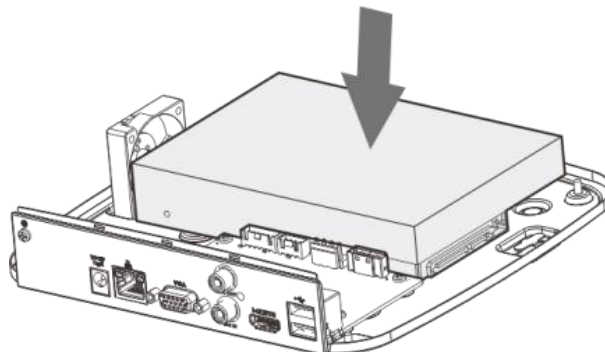
Figure 1-3 Installing HDD (3)
