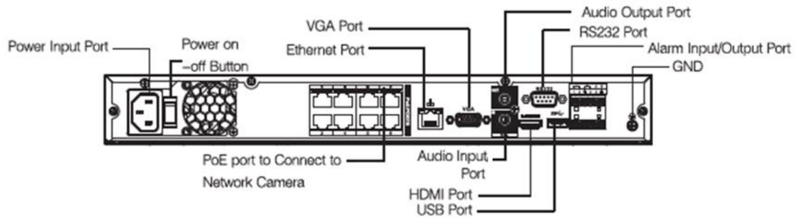
Figure 2-1 1U series connection
