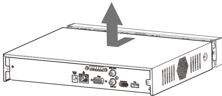
Figure 2-8 Installing HDD (2)
